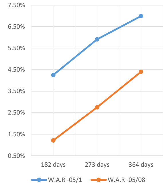
Graph 1.0 – yield curve showing movement in T-bills between Jan and early August 2022
